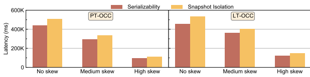
Figure 15: Snapshot transactions
